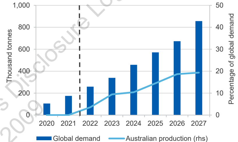
Figure 15.7: World and Australian lithium hydroxide output
