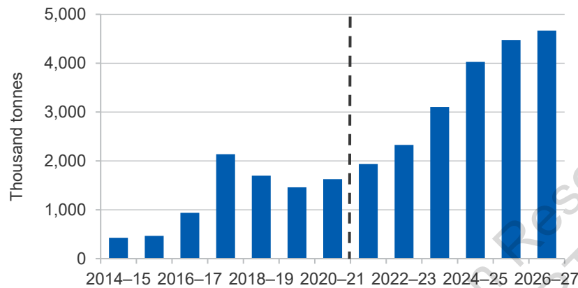
Figure 15.6: Spodumene production
