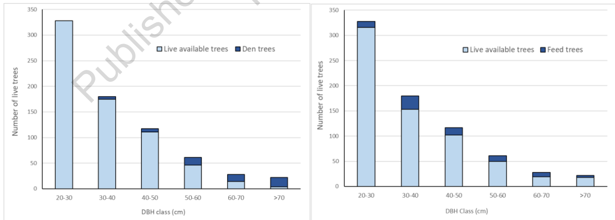
Figure 5 Size of live trees used by greater gliders for denning and foraging
